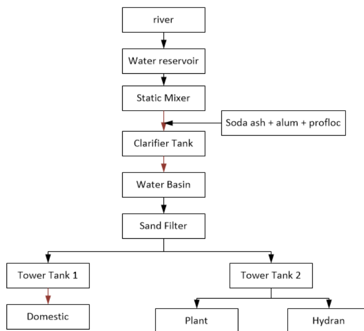
Figure 1. Water treatment process flow diagram of the mill
