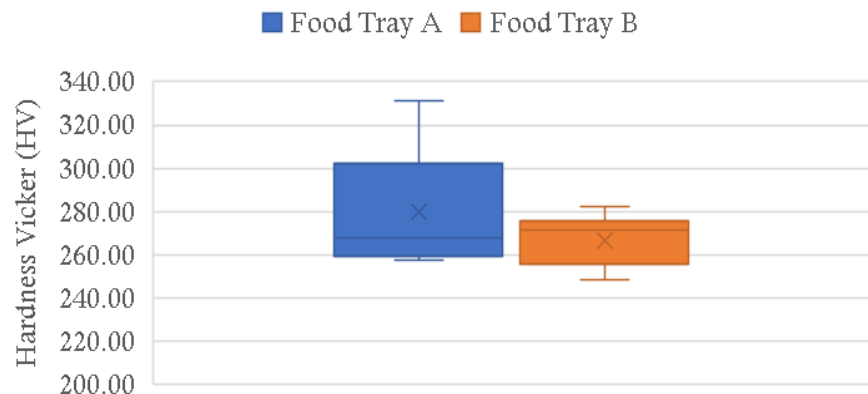
Figure 4. Boxplot of Microvicker hardness values for Food tray A and Food tray B
