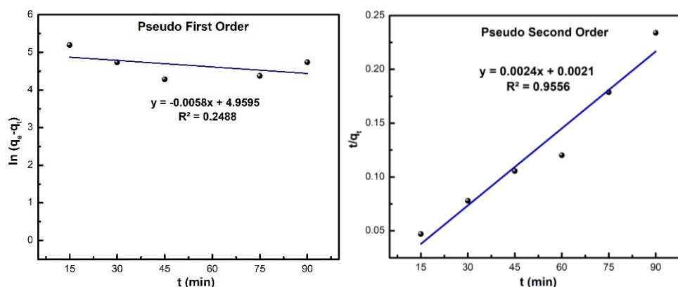
Figure 6. Adsorption Kinetics Graph (PFO and PSO)
