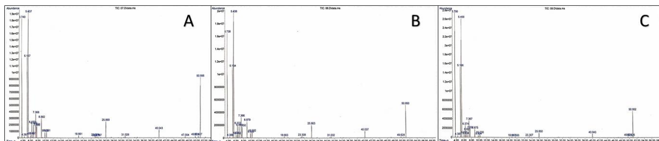
Figure 3. GC Chromatogram of Banda Variety Nutmeg ( Myristica fragrans Houtt.) Seed Essential Oil from a) Banda; b) Titawaai; c) Seith
