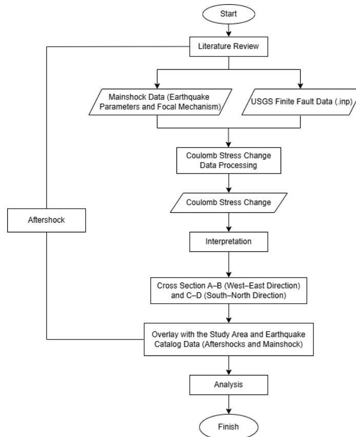
Figure 2. Research Workflow
