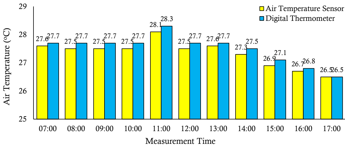
Figure 2. Comparison of DHT11 Air Temperature Sensor and Digital Thermometer
