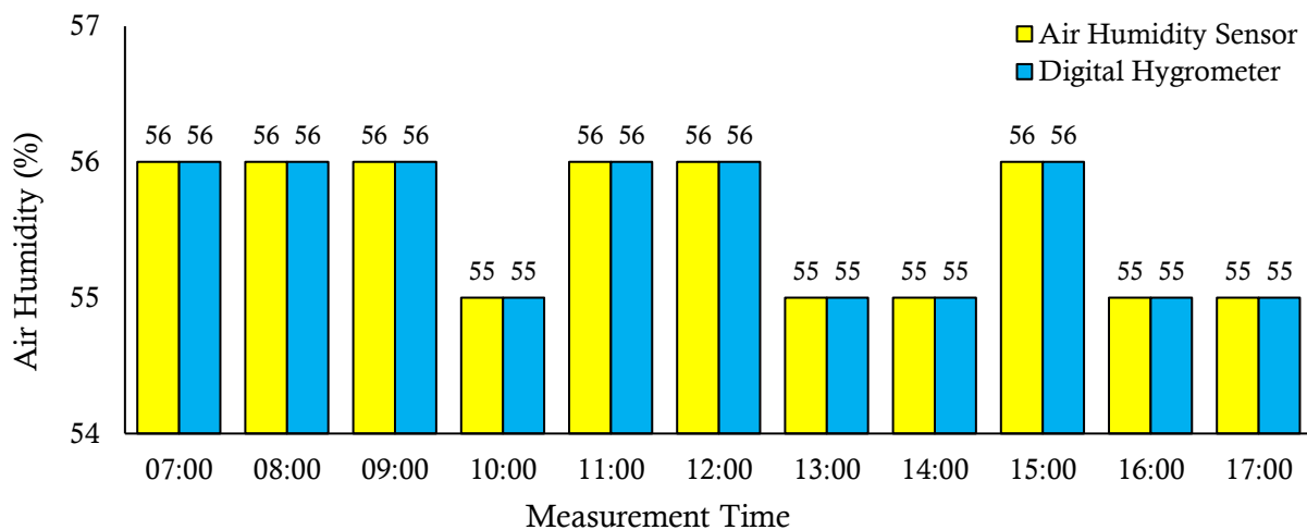
Figure 3. Comparison of DHT11 Air Humidity Sensor and Digital Hygrometer
