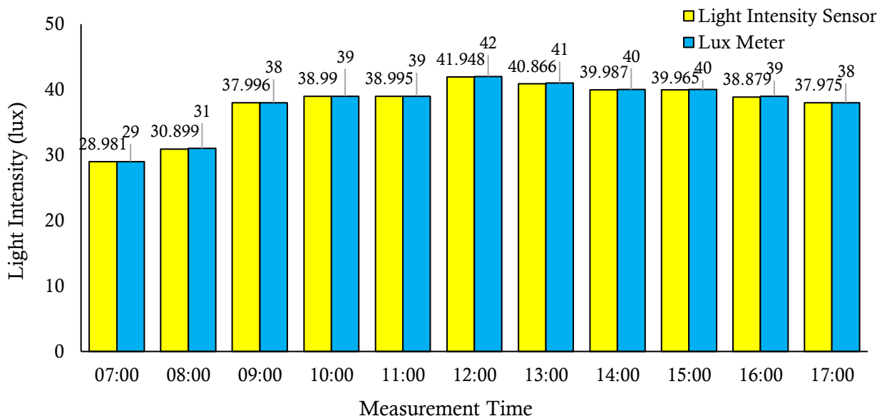
Figure 4. Comparison of BH1750 Light Intensity Sensor and Lux Meter
